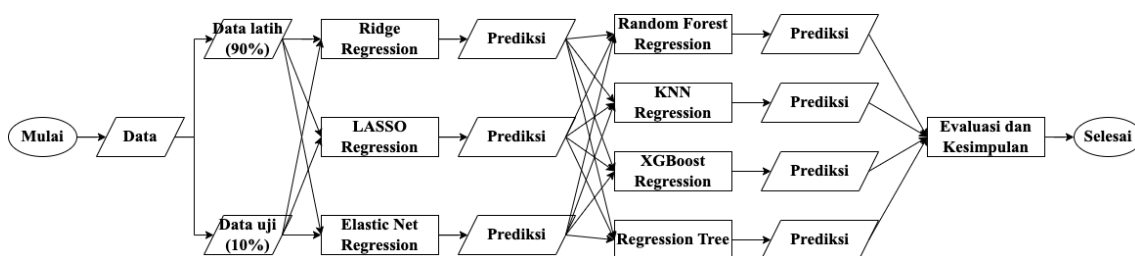
Gambar 2. Alur penelitian
